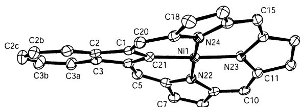
Figure 7. ORTEP III drawing (50% probability level) of 14b , depicting the presence of a ruffled conformation; hydrogen atoms and core substituents have been omitted for clarity. Selected bond lengths (Å): C(21)–Ni 1.896(3), N(22)–Ni 1.934(2), N(23)–Ni 1.964(2), N(24)–Ni 1.928(2), C(1)–C(21) 1.417(4), C(4)–C(21) 1.426(4). Selected bond angles (deg): C(21)–C(1)–C(2) 110.6(3), C(1)C(2)–C(3) 106.5(3), C(2)–C(3)–C(4) 106.8(3), C(3)–C(4)–C(21) 110.6(3), C(4)–C(21)–C(1) 105.3(2), C(6)–N(22)–C(9) 104.7(2), C(11)–N(23)–C(14) 105.3(2), C(16)–N(24)–C(19) 104.6(2), C(21)–Ni–N(22) 90.4(1), N(22)–Ni–N(23) 90.1(1), N(23)–Ni–N(24) 89.9(1), N(24)–Ni–C(21) 89.9(1), C(21)–Ni–N(23) 177.2(1), N(22)–Ni–N(24) 176.2(1).
