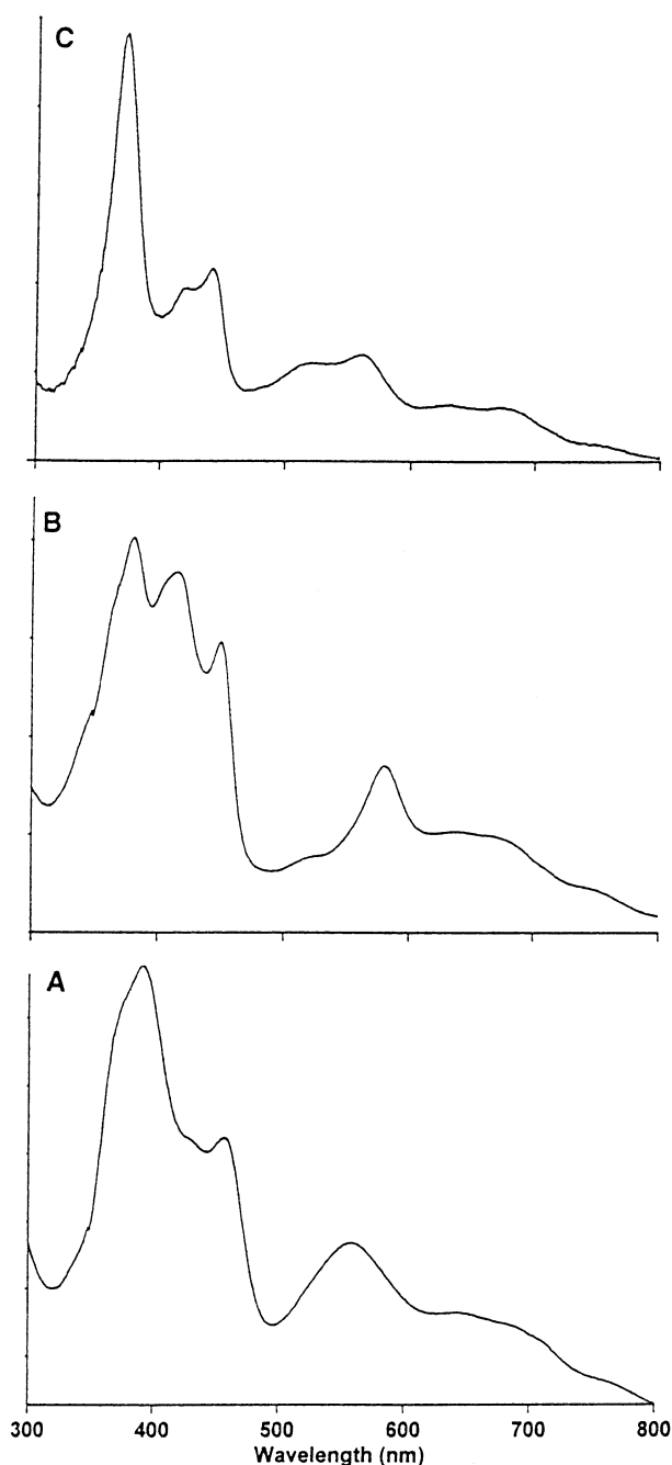
Figure 1. UV-vis absorption spectra of metalloazuliporphyrins in chloroform: (A) nickel(II) complex 14b ; (B) palladium(II) complex 15b ; (C) platinum(II) complex 16b .
