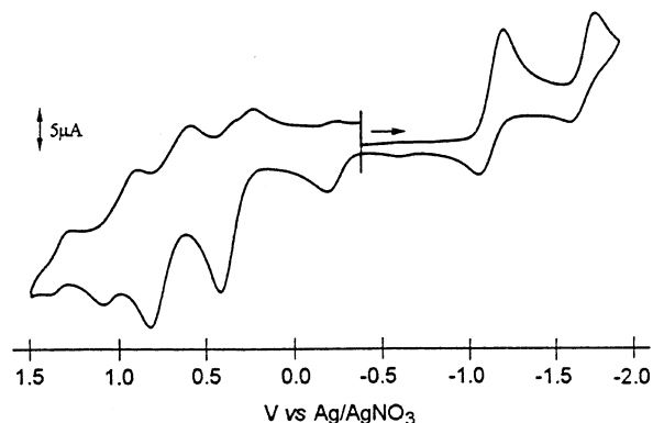
Figure 5. Cyclic voltammogram (200 mV/s) of 13a in anhydrous dichloromethane, 0.2 M \text{Bu}_4\text{NBF}_4 .
