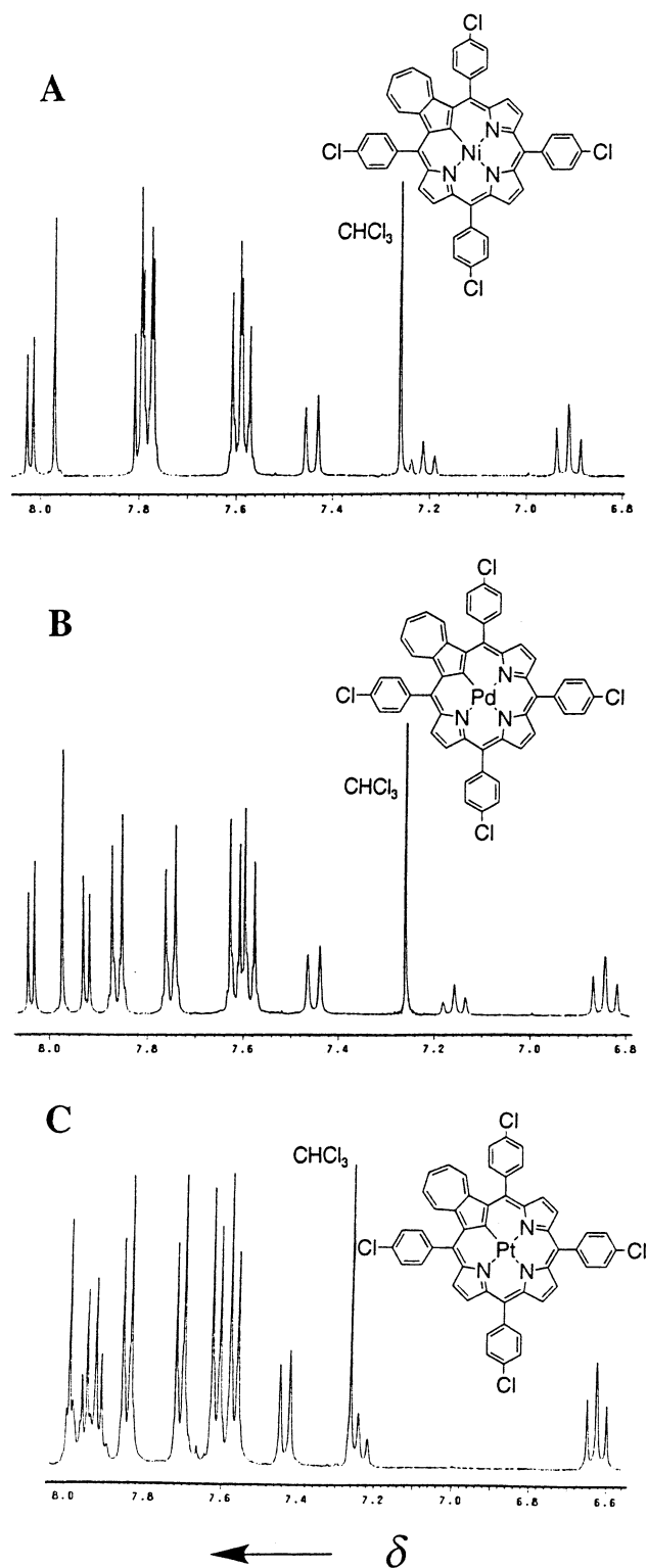
Figure 4. 400 MHz proton NMR spectrum of tetrakis(4-chlorophenyl)-azuloporphyrin chelates in \text{CDCl}_3 : (A) nickel(II) complex 17b ; (B) palladium(II) complex 18b ; (C) platinum(II) complex 19b . In the spectrum for 19b , the ^{195}\text{Pt} satellite peaks for the pyrrolic protons are clearly evident between 7.9 and 8.0 ppm.
