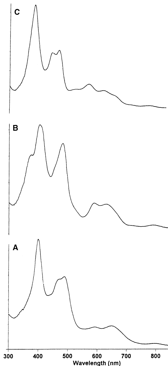
Figure 3. UV-vis absorption spectra of tetrakis(4-chlorophenyl)azuliporphyrin chelates in chloroform: (A) nickel(II) complex 17b ; (B) palladium(II) complex 18b ; (C) platinum(II) complex 19b .
